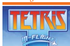
In-Flight Tetris®
