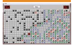
Mine Sweeper
