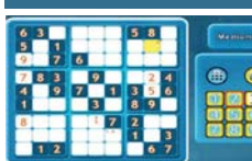
In-Flight Sudoku
